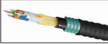
Optical Fiber Loose Tube Cable, Outdoor
